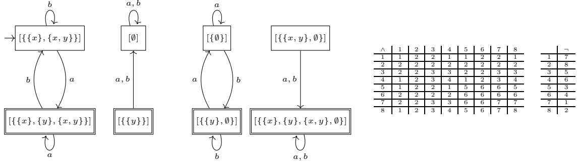
Figure 4.4: The minimal CABA-structured DFA for L = (a + b)^*a , where 1 \equiv [\{\{x\}, \{x, y\}\}] , 2 \equiv [\emptyset] , 3 \equiv [\{\emptyset\}] , 4 \equiv [\{\{x, y\}, \emptyset\}] , 5 \equiv [\{\{x\}, \{y\}, \{x, y\}\}] , 6 \equiv [\{\{y\}\}] , 7 \equiv [\{\{y\}, \emptyset\}] , 8 \equiv [\{\{x\}, \{y\}, \{x, y\}, \emptyset\}]
