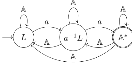
Figure 4.7: The orbit-finite representation of the canonical nominal RFSa for L = \{vawau \mid v, w, u \in \mathbb{A}^*, a \in \mathbb{A}\}
