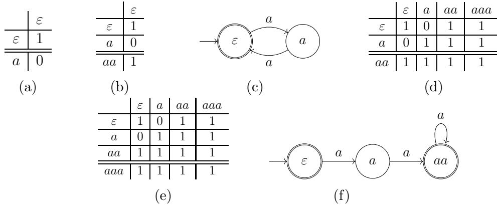
Figure 1.2: An example run of (a variation of) Angluin’s L^* algorithm for the target regular language 1 + a \cdot a \cdot a^* = \{\varepsilon, aa, aaa, \dots\} \subseteq \{a\}^*
