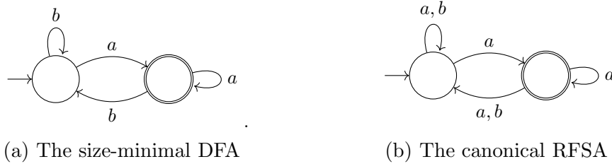
Figure 1.5: Two canonical acceptors for (a + b)^*a
