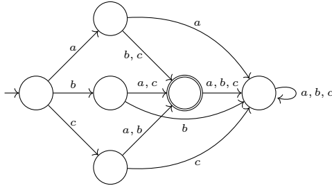
Figure 1.1: Up to isomorphism, the unique size-minimal DFA accepting the language \{ab, ac, ba, bc, ca, cb\} \subseteq \{a, b, c\}^* [20]
