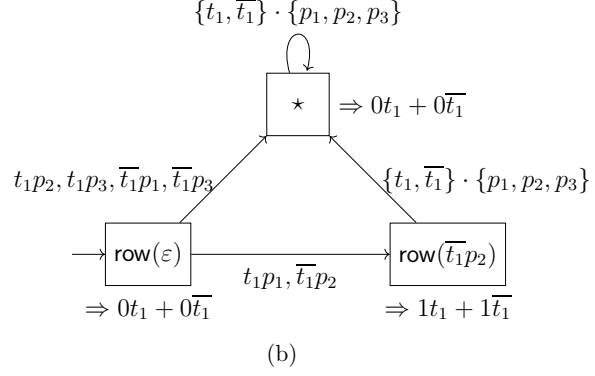
Figure 3.8: For e = \text{if } t_1 \text{ then do } p_1 \text{ else do } p_2 , |\Sigma| = 3 , and |T| = 2 , our implementation of \text{GL}^* accepts the table in (a), which induces the automaton in (b).
