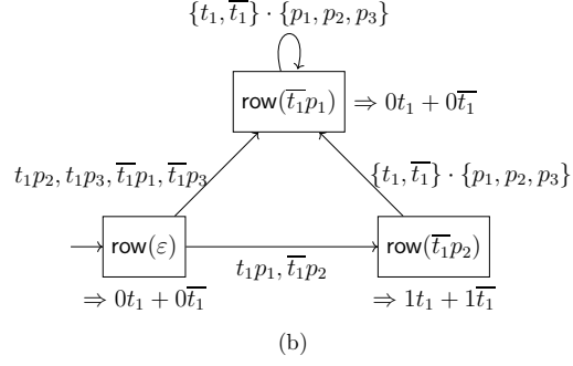
Figure 3.9: For e = \text{if } t_1 \text{ then do } p_1 \text{ else do } p_2 , |\Sigma| = 3 , and |T| = 2 , our implementation of L^* accepts the table in (a), which induces the automaton in (b).
