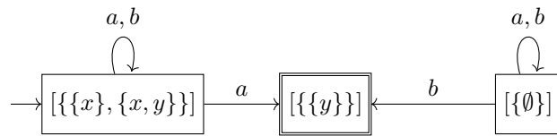
Figure 4.5: The átomaton for L = (a + b)^*a
