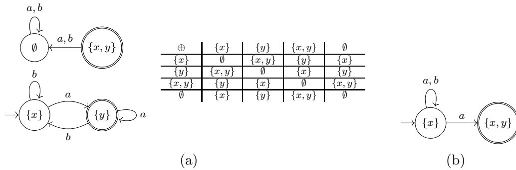
Figure 4.8: (a) The minimal \mathbb{Z}_2 -vector space structured DFA for L = (a+b)^*a (freely-generated by the DFA in Figure 4.3); (b) Up to the choice of a basis, the minimal xor automaton for L = (a + b)^*a
