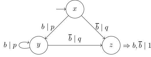
Figure 3.4: The Thompson-automaton \mathcal{X}_{p^{(b)}q} for T = \{b\} and \Sigma = \{p, q\}
