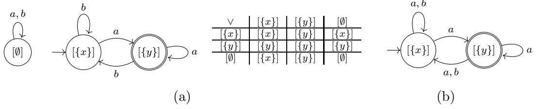
Figure 4.6: (a) The minimal CSL-structured DFA for L = (a+b)^*a ; (b) The canonical RFSA for L = (a+b)^*a
