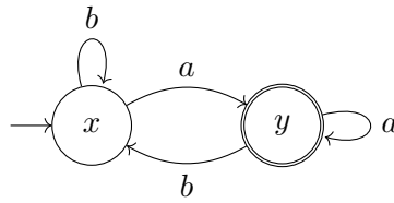
Figure 4.3: The minimal DFA for L = (a + b)^*a
