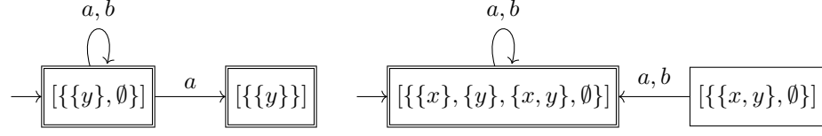
Figure 4.11: The minimal xor-CABA automaton for L = (a + b)^*a
