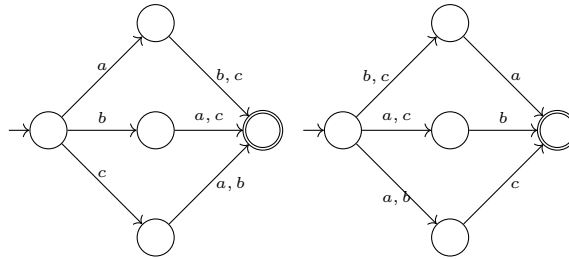
Figure 4.1: Two non-isomorphic size-minimal NFA accepting the language \{ab, ac, ba, bc, ca, cb\} \subseteq \{a, b, c\}^* [20]
