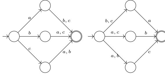
Figure 1.4: Two non-isomorphic size-minimal NFA accepting the language \{ab, ac, ba, bc, ca, cb\} \subseteq \{a, b, c\}^* [20]
