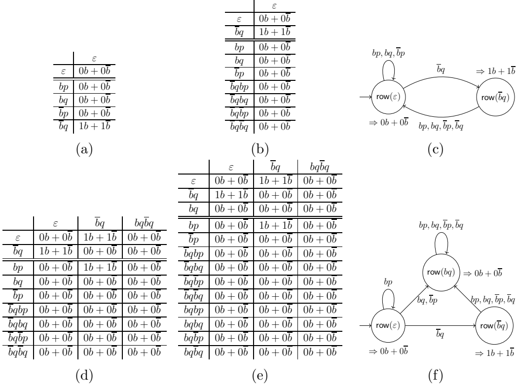
Figure 3.1: An example run of Angluin’s L^* algorithm for the target language \llbracket(\text{while } b \text{ do } p); q\rrbracket
