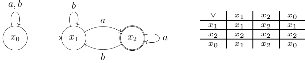
Figure 1.8: The minimal CSL-structured DFA accepting (a + b)^*a \subseteq \{a, b\}^*
