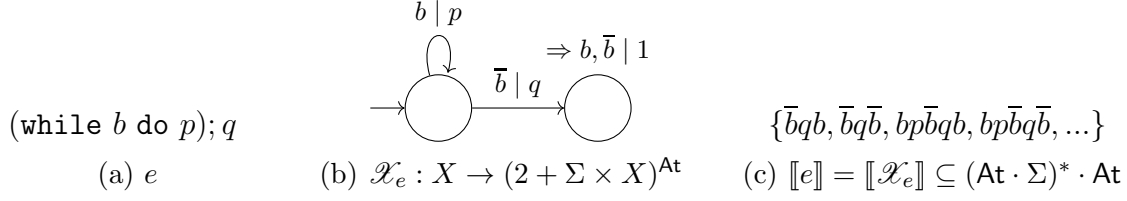
Figure 1.3: The interplay between expressions, automata, and languages in GKAT, for \Sigma = \{p, q\} and \text{At} = \{b, \bar{b}\}
