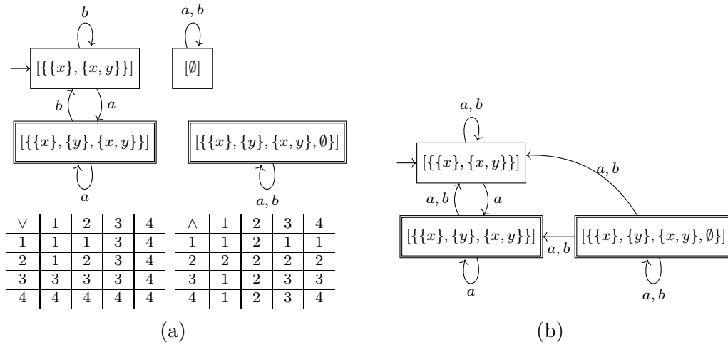
Figure 4.9: (a) The minimal CDL-structured DFA for L = (a + b)^*a , where 1 \equiv [\{\{x\}, \{x, y\}\}] , 2 \equiv [\emptyset] , 3 \equiv [\{\{x\}, \{y\}, \{x, y\}\}] , 4 \equiv [\{\{x\}, \{y\}, \{x, y\}, \emptyset\}] ; (b) The distromaton for L = (a + b)^*a
