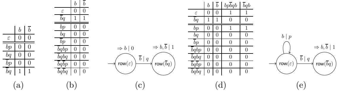
Figure 3.2: An example run of \text{GL}^* for the target language \llbracket(\text{while } b \text{ do } p); q\rrbracket
